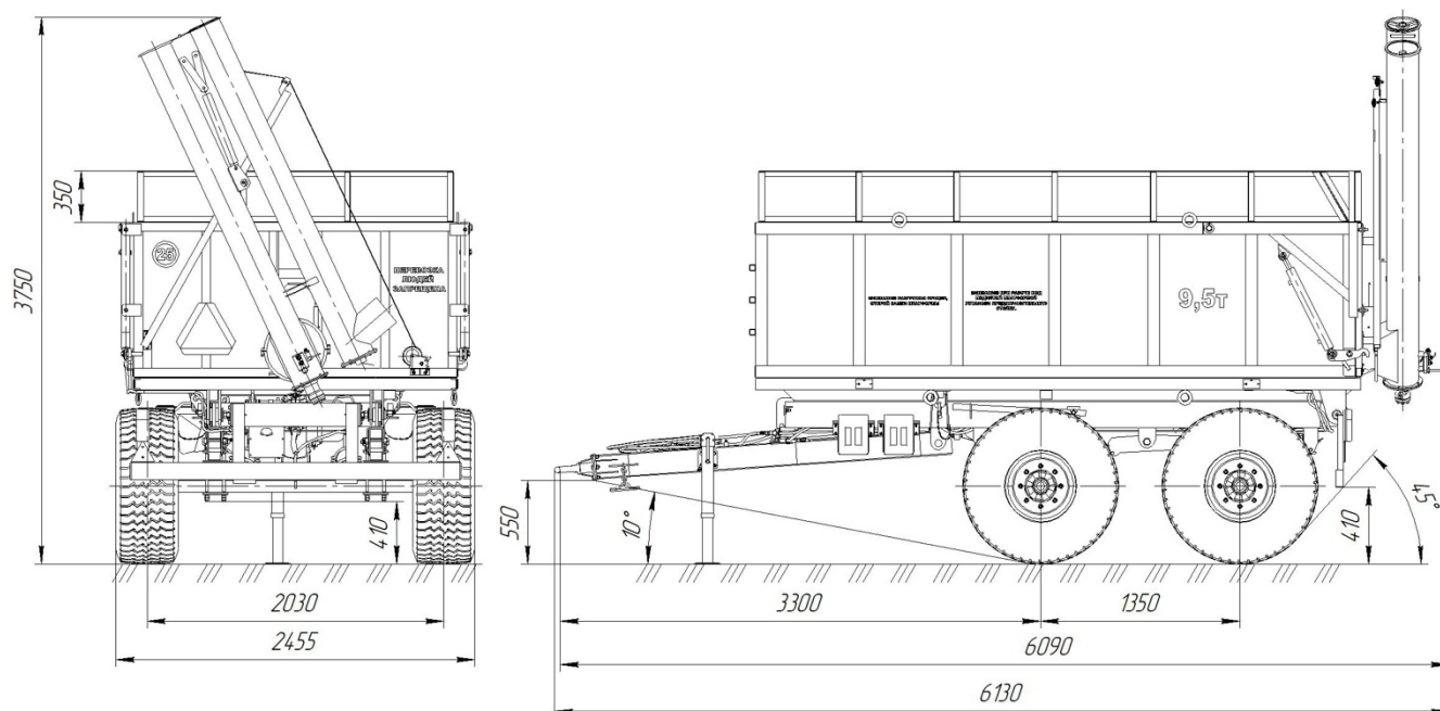
Image 1.4 – Semi-trailer version PTS-9NP
