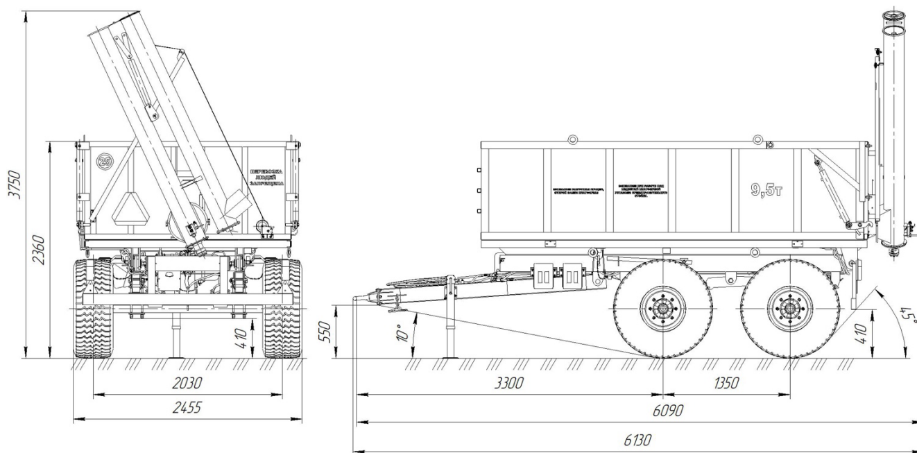
Image 1.3 – Semi-trailer version PTS-9P
